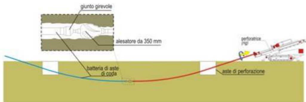
Figura 14 Alesatura (back reaming)
